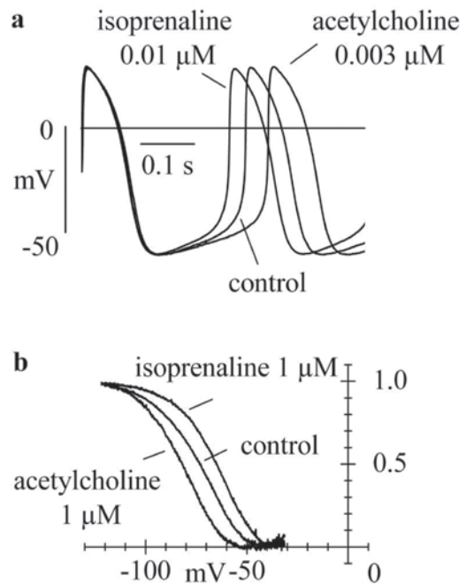
FIGURE 2. I_f mediates the modulation of cardiac rate by the autonomic nervous system. a , spontaneous activity recorded from a SAN myocyte; activity is accelerated by isoprenaline and slowed by acetylcholine, and rate changes do not involve changes of action potential shape or duration but are only associated to changes in the slope of diastolic depolarization. b , the I_f activation curve shifts to the right in the presence of isoprenaline and to the left in the presence of acetylcholine, thus increasing and decreasing, respectively, the current activated at each voltage; these effects are responsible for the changes of diastolic depolarization rate shown in panel a. [Modified with permission from DiFrancesco, 1993 (a) and Accili et al., 1997 (b)].
