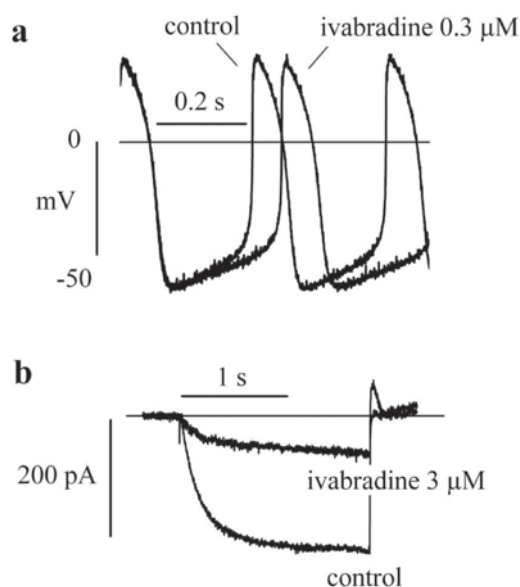
FIGURE 3. Ivabradine slows pacemaker rate and blocks f-channels. a, spontaneous activity recorded from a single SAN myocyte is slowed by ivabradine 0.3 \mu M, through a decreased rate of diastolic depolarization. b, ivabradine-induced block of I_f recorded during repetitive activating/deactivating steps (-100/+5 mV) applied every 6 s from a holding potential of -35 mV.
